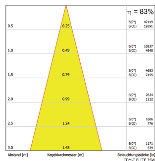
Kegeldiagramm | NFL 24,0°
